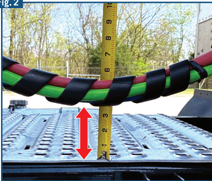
Fig. 2. 3-6" deck clearance is recommended when connected.
